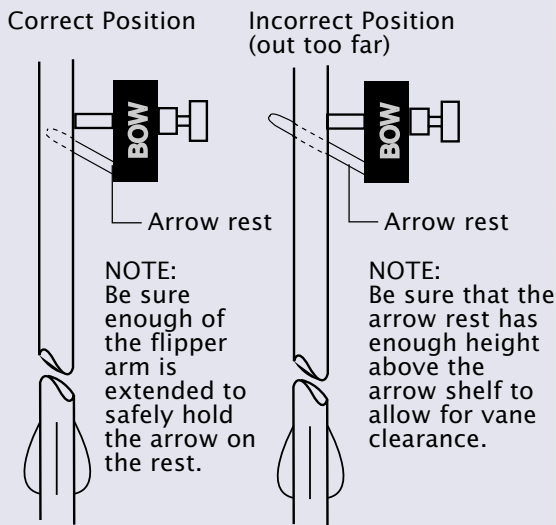
Fig. 9 Arrow Rest - Back View, Vane Clearance (CR)
