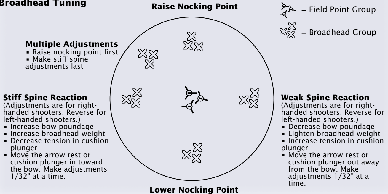
Fig. 20 Broadhead Tuning
